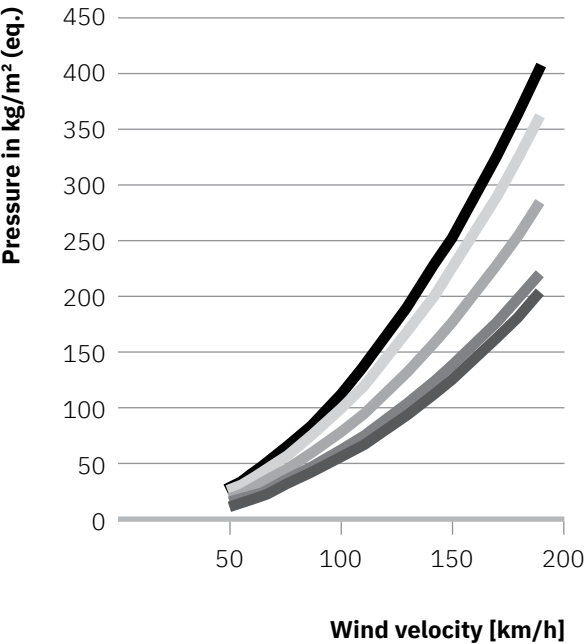
WIND SPEED/PRESSURE BASIC PRESSURE ACCORDING TO STANDARD EN 1991-1-4
