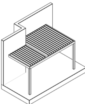
TYPE 8 Wall-mounted blades perpendicular to wall
